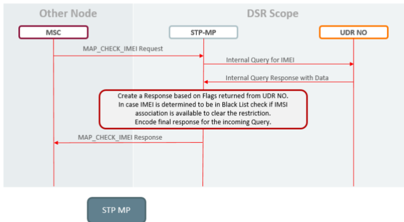
Figure 81 – SS7 EIR call flow
