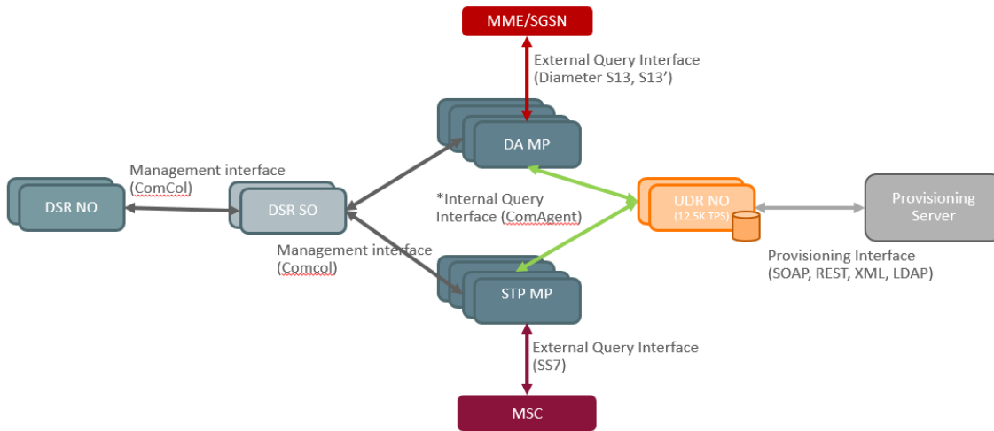
Figure 80 – EIR solution architecture.
