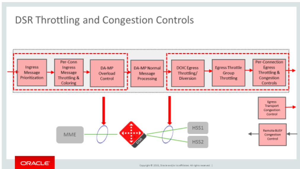
Figure 21 - Congestion Control
