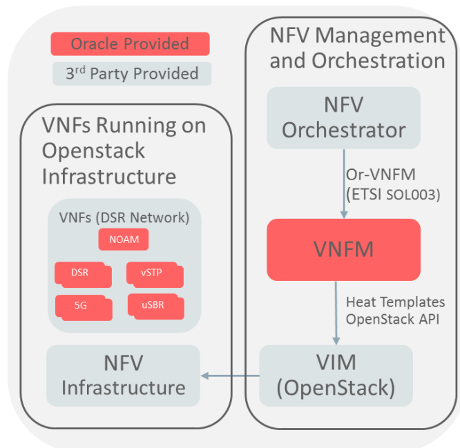
Figure 72 – DSR VNFM
