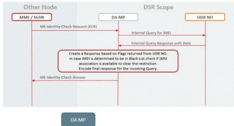
Figure 82 – S13 EIR Call Flow
